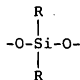
bifunctional
