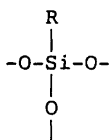
trifunctional
