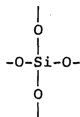
tetrafunctional
