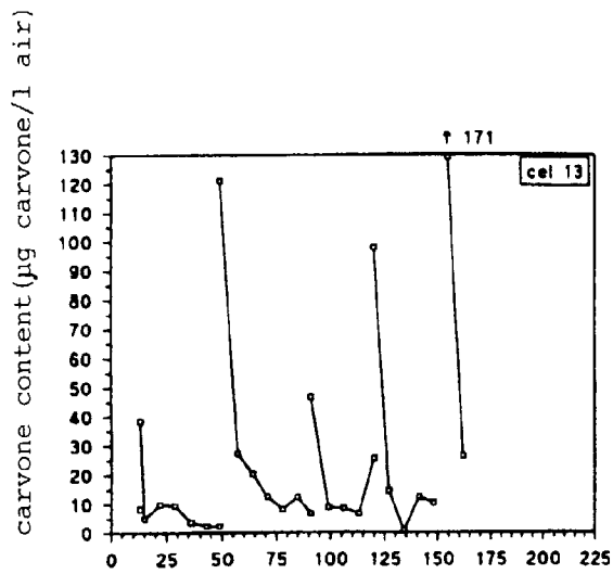
FIG. 1 storage period (days)
