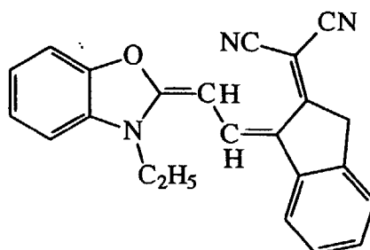
Dye P-2 \lambda_{\text{max}} = 571 \text{ nm} (acetone)
