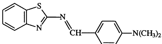
Dye P-3 "GY-9" from U.S. Patent 4,812,439 \lambda_{\text{max}} = 410 \text{ nm} (acetone)
