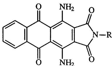
Cyan Dye C-2 "Kayaset B-766", Disperse Blue 60 R = C_3H_6OCH_3 \text{ or } C_2H_5OCH_3
