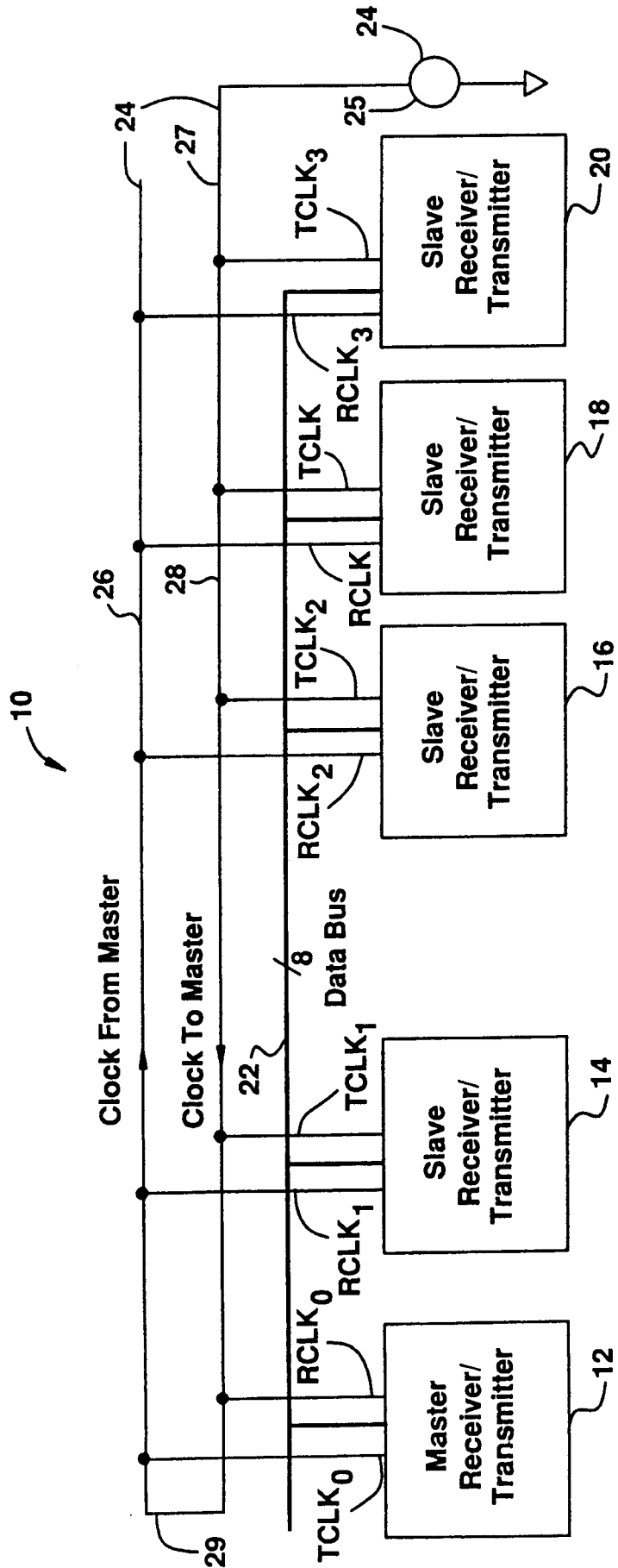
FIG. 1 PRIOR ART
