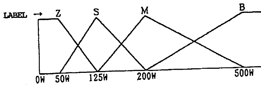
Fig. 11 (LOAD VALUE)
