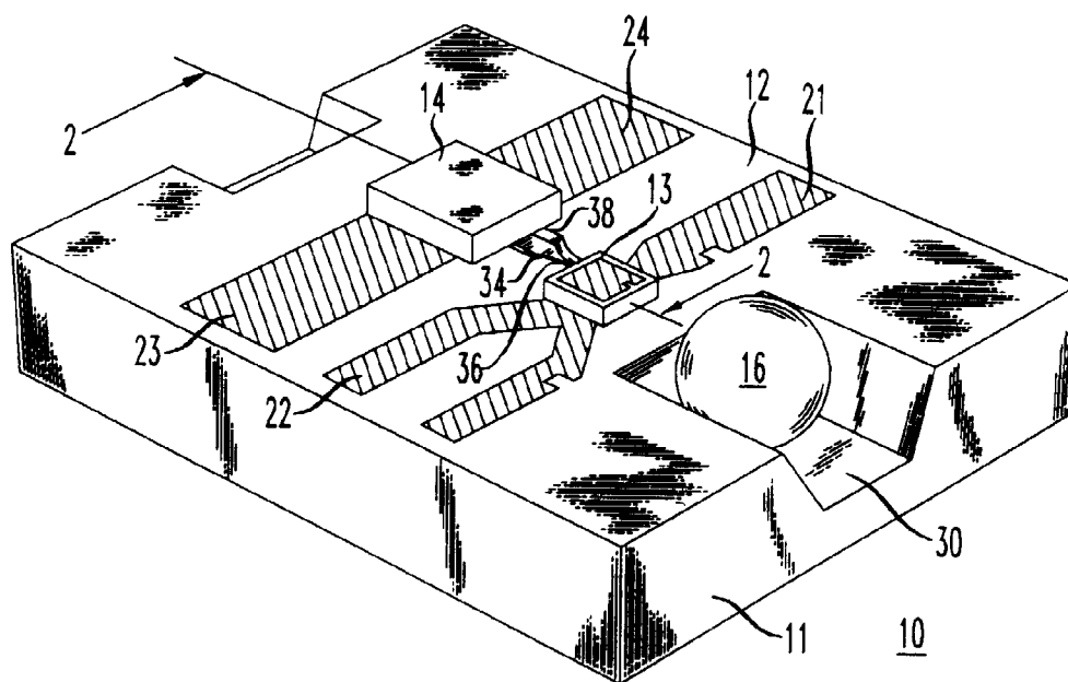
FIG. 1 (PRIOR ART)
