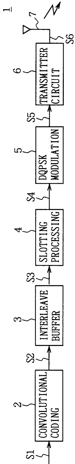
FIG. 2A (RELATED ART)
