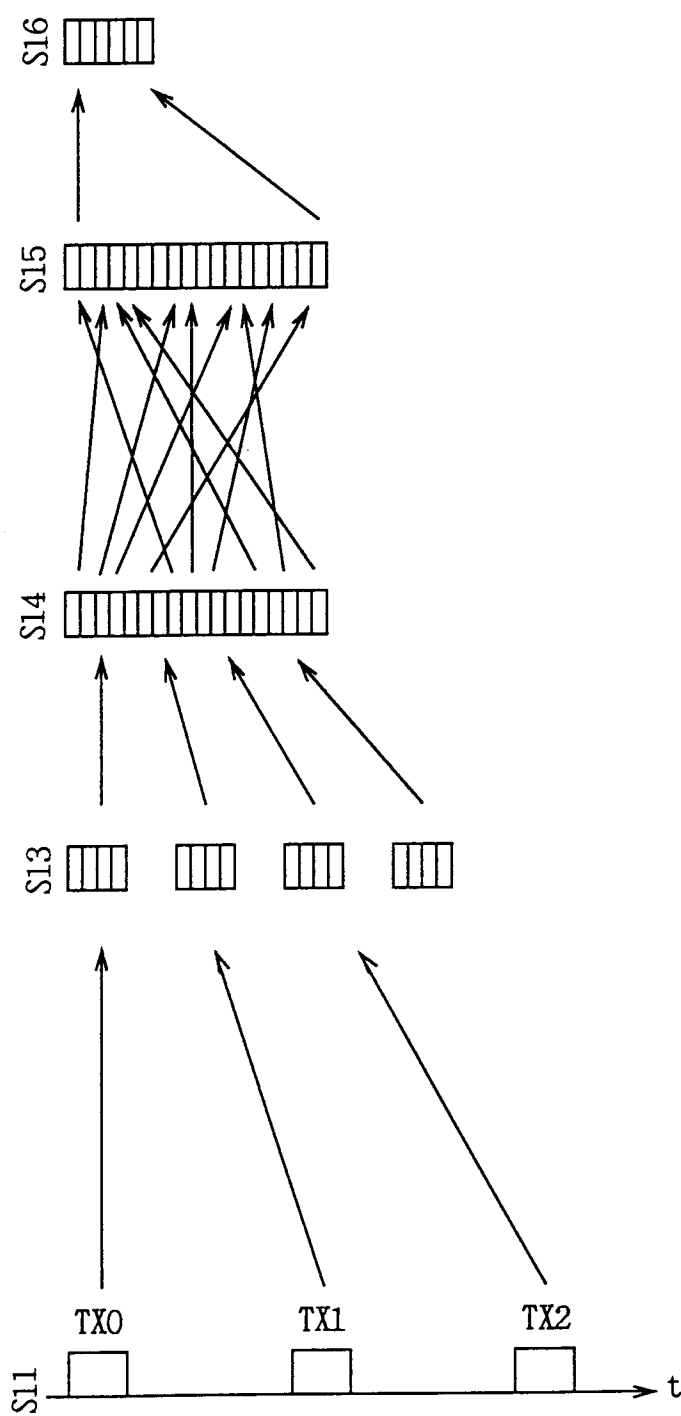
FIG. 3B (RELATED ART)
