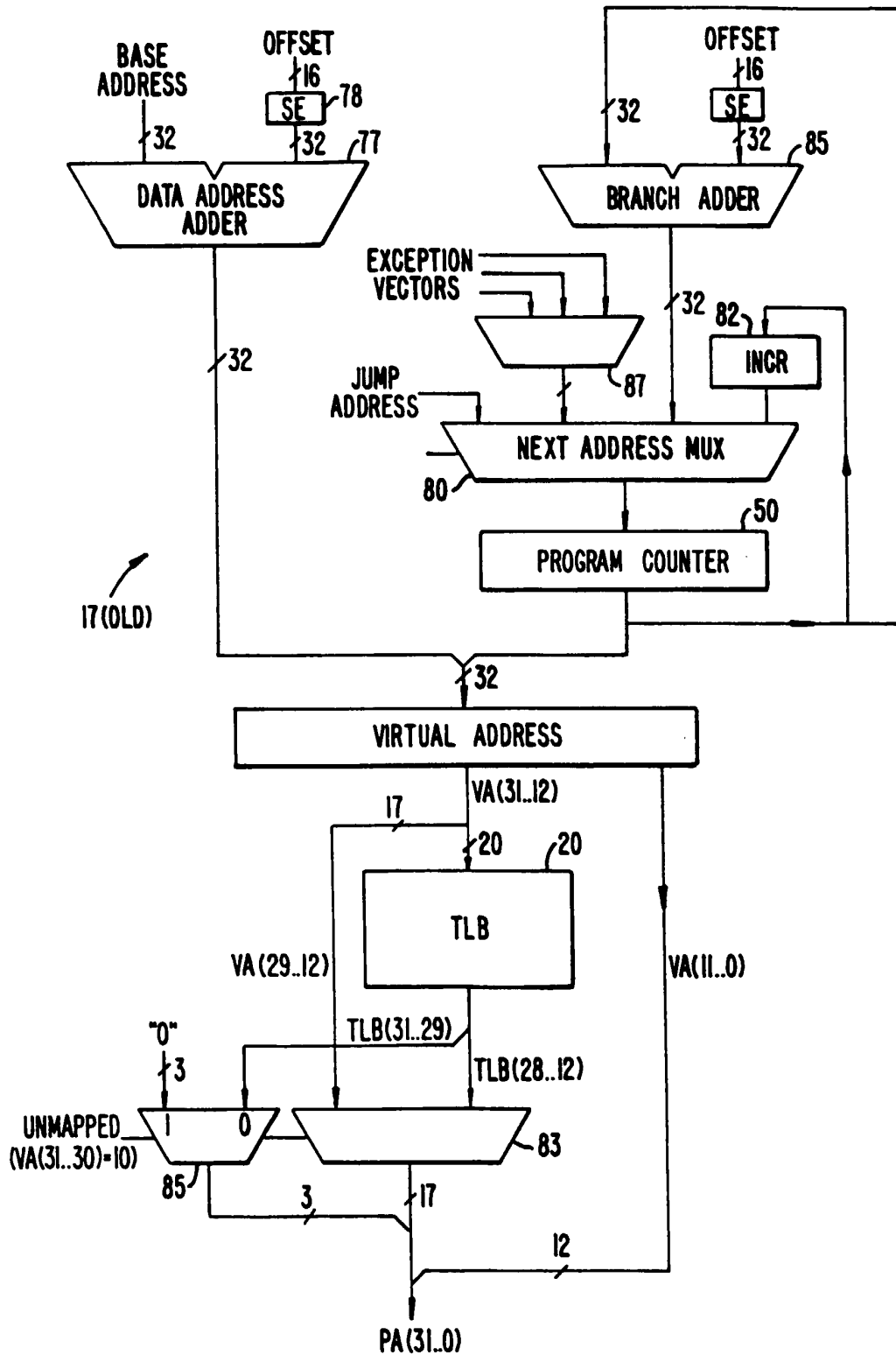
FIG. 3C. (PRIOR ART)
