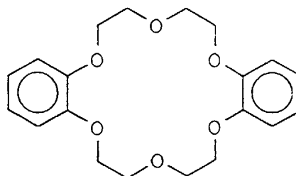
dibenzo-18-crown-6 of formula (A)
