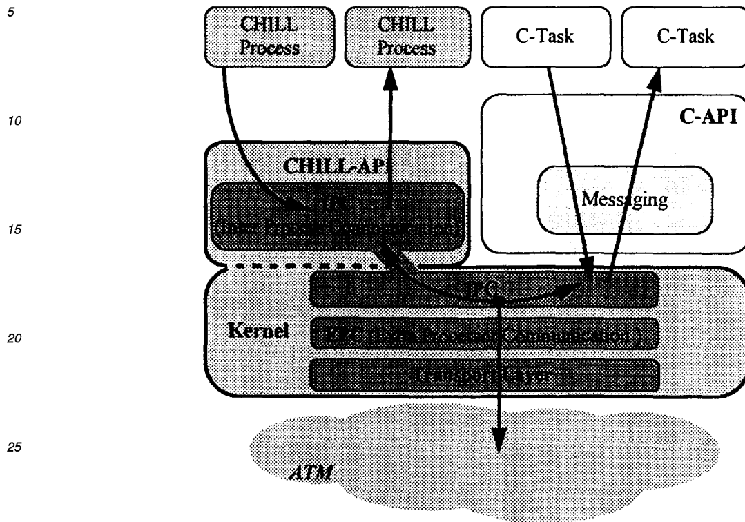
Figure 4: Communication Architecture
