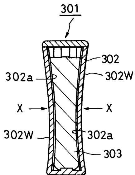
FIG. 16 PRIOR ART
