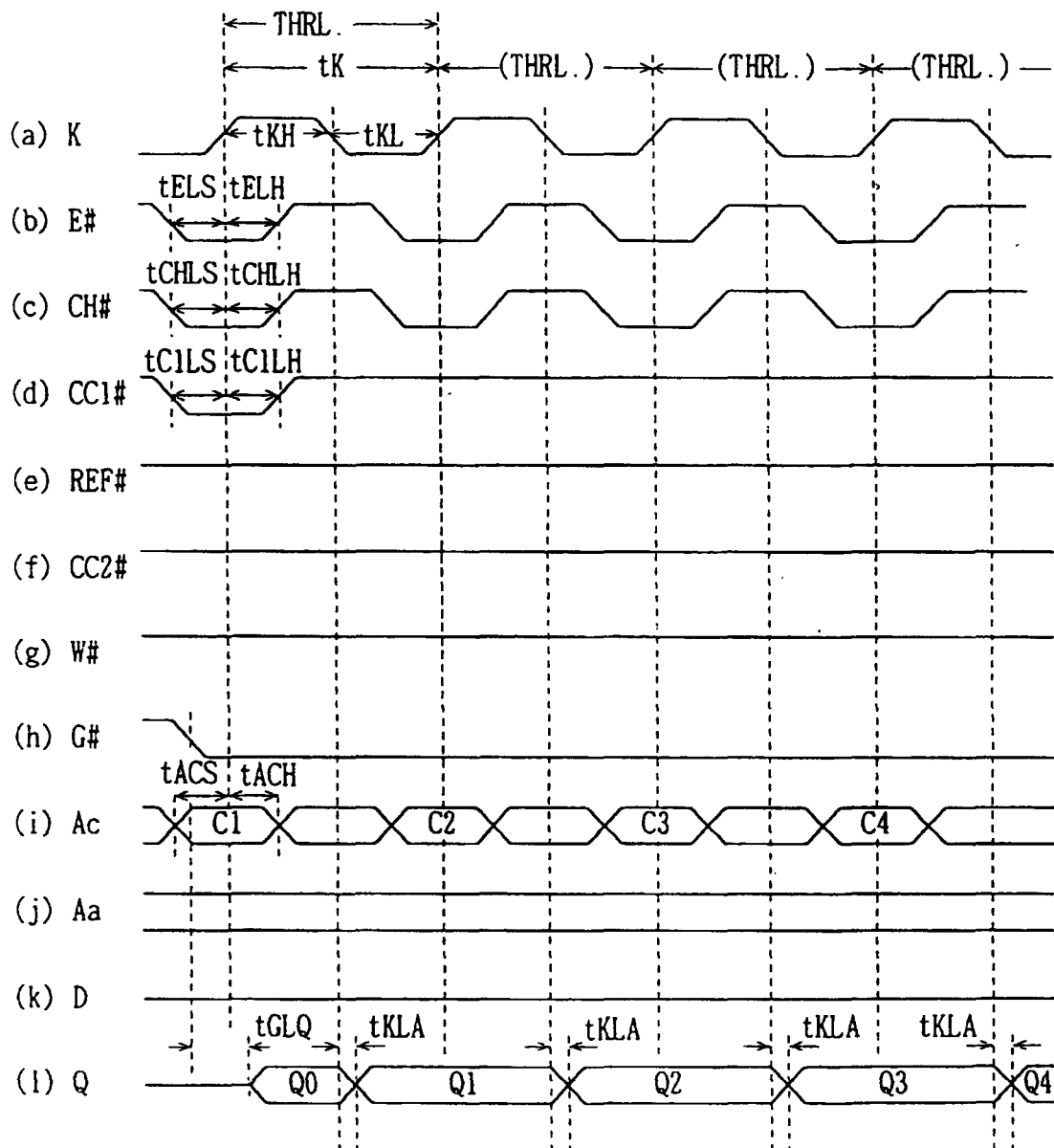
F I G. 1 4 0 THRL: CACHE HIT READ OPERATION (HIGH SPEED OPERATION) (LATCH OUTPUT)
