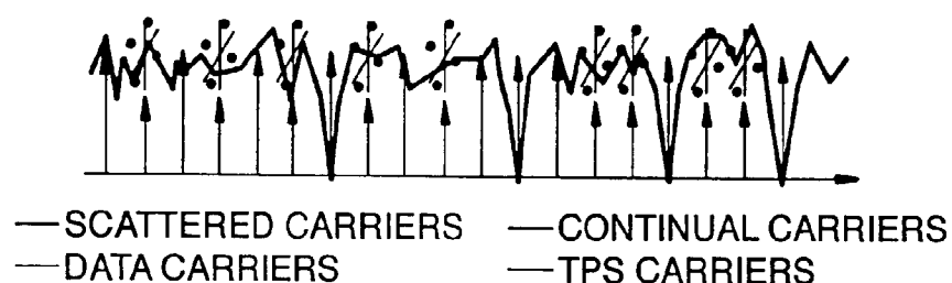
FIG. F4B VALUE OF THE SECOND PHASE DIFFERENCE AT EACH CARRIER
