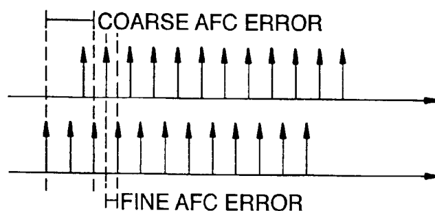
FIG. F4A COARSE AND FINE FREQUENCY OFFSET
