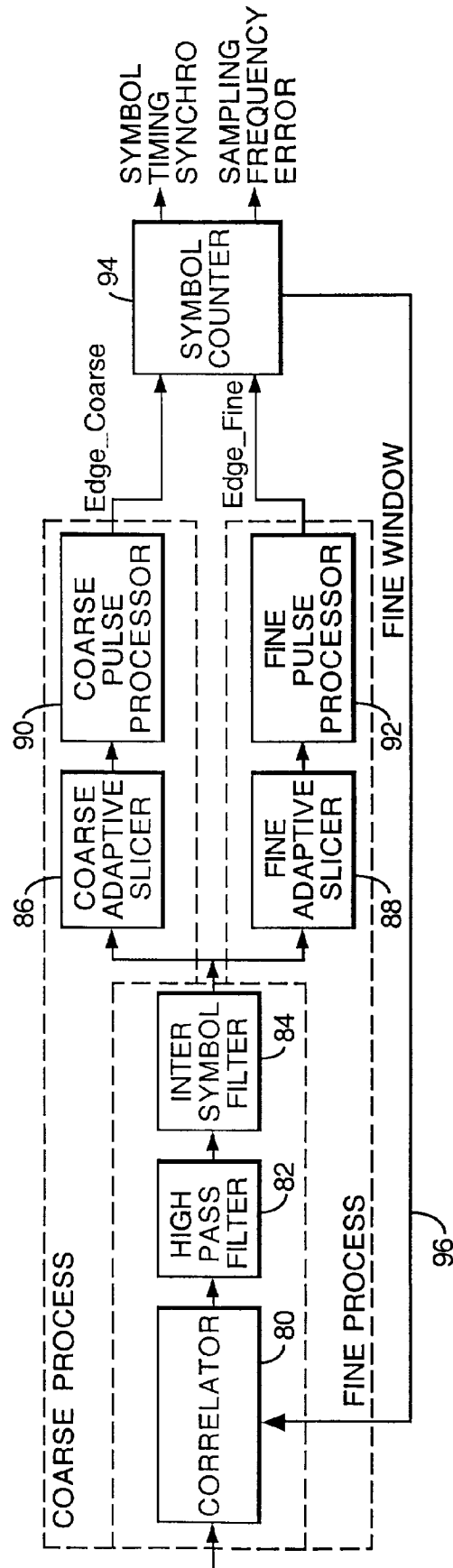
FIG. C9 SUB-SAMPLING IMPLEMENTATION OF THE TIMING SYNCHRONISATION
