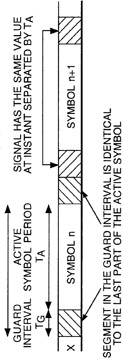
FIG. D4 OFDM SYMBOL COMPRISING ITS ACTIVE AND GUARD INTERVAL AND THEIR RELATIONSHIP
