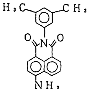
SOLVENT YELLOW 44
