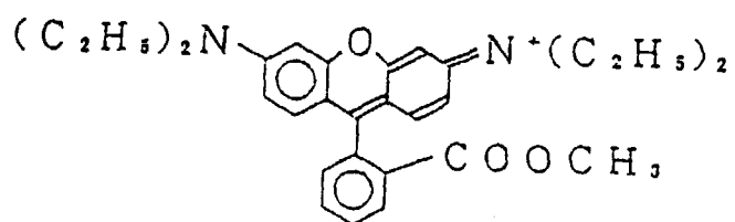
BASIC VIOLET 11
