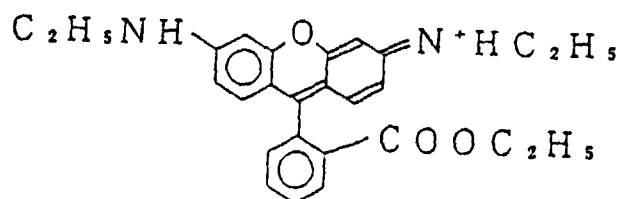
BASIC RED 1
