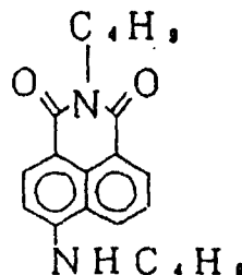
SOLVENT YELLOW 116
