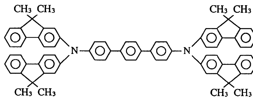
Compound 46
