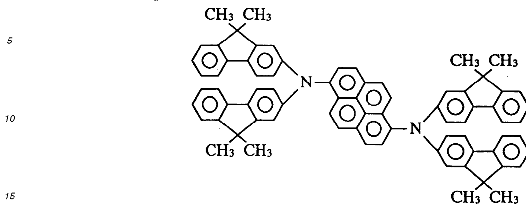
Compound 70
