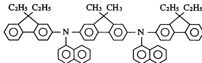
Compound 15
