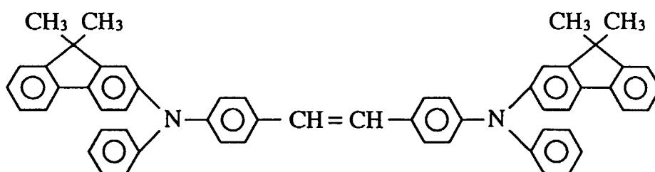
Compound 29
