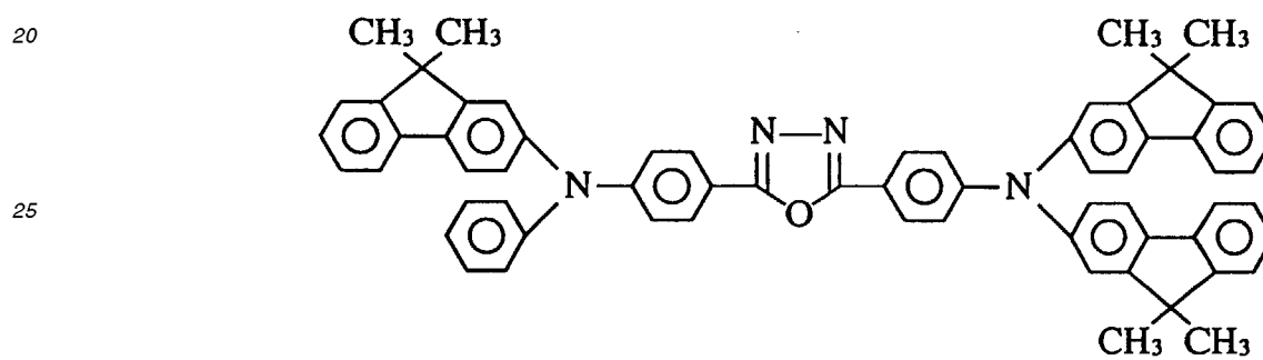
Compound 99
