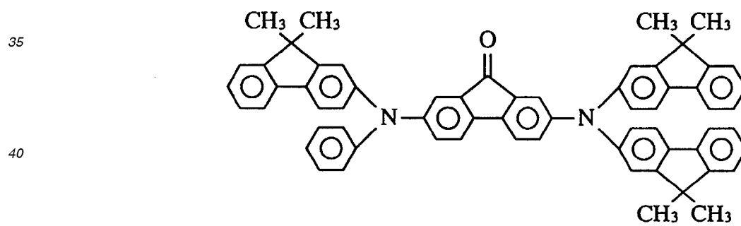
Compound 100
