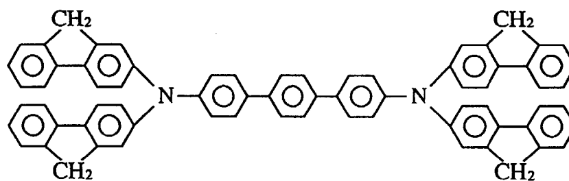
Compound 45
