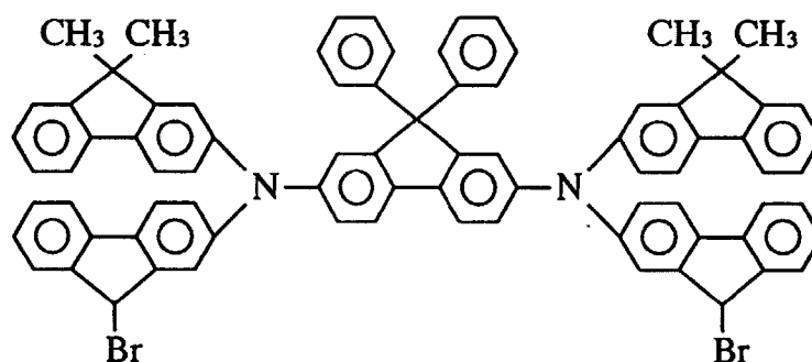
Compound 52
