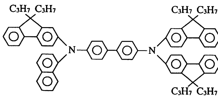
Compound 91
