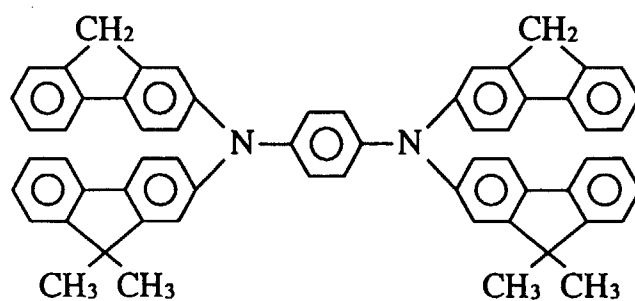
Compound 37
