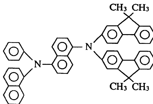
Compound 86
