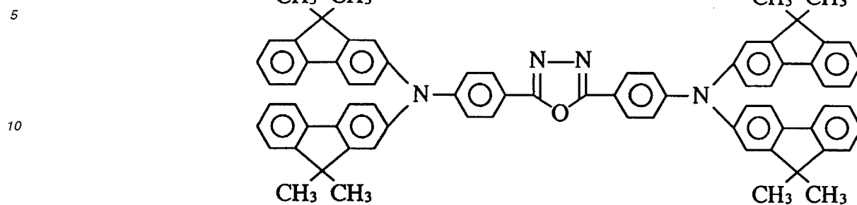
Compound 59
