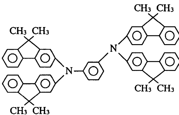
Compound 36
