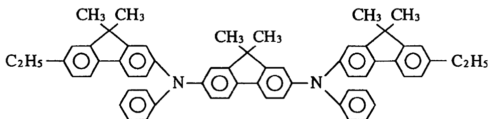
Compound 21
