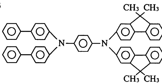
Compound 73
