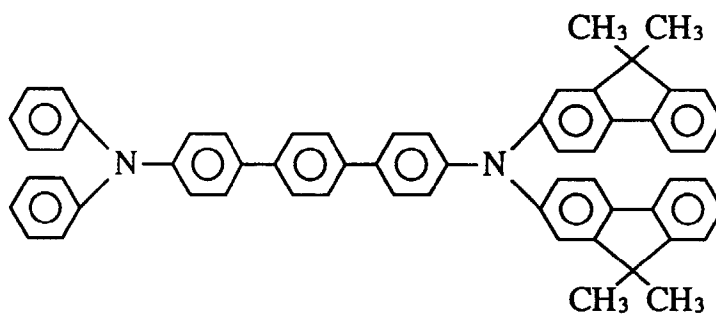
Compound 77
