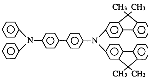
Compound 74
