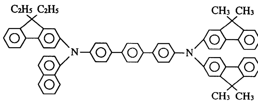
Compound 94
