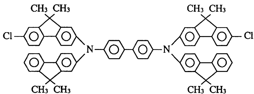
Compound 43
