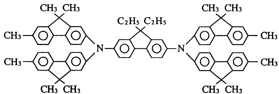
Compound 51
