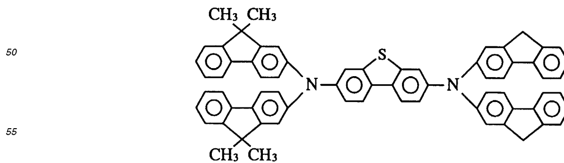
Compound 66
