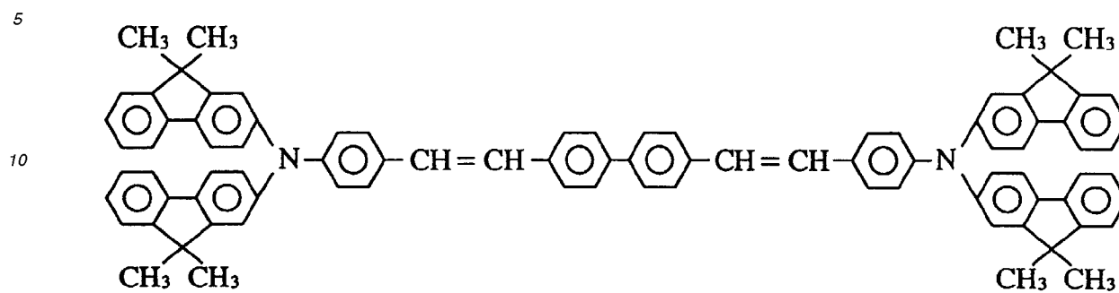
Compound 67
