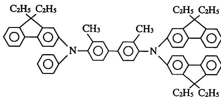
Compound 92
