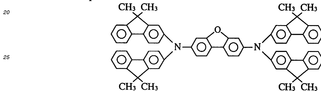
Compound 68
