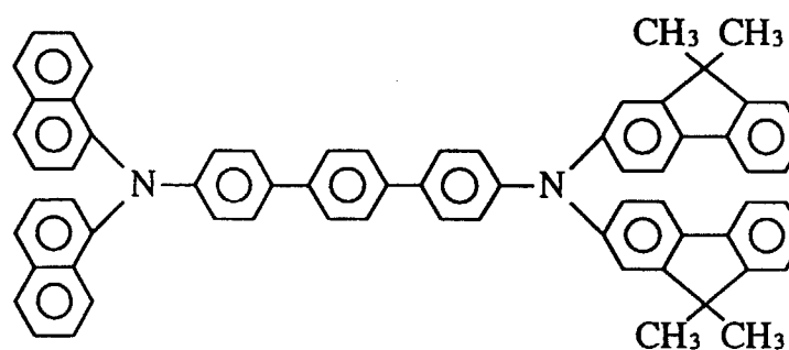
Compound 78
