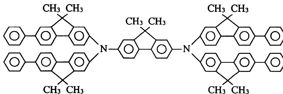
Compound 53
