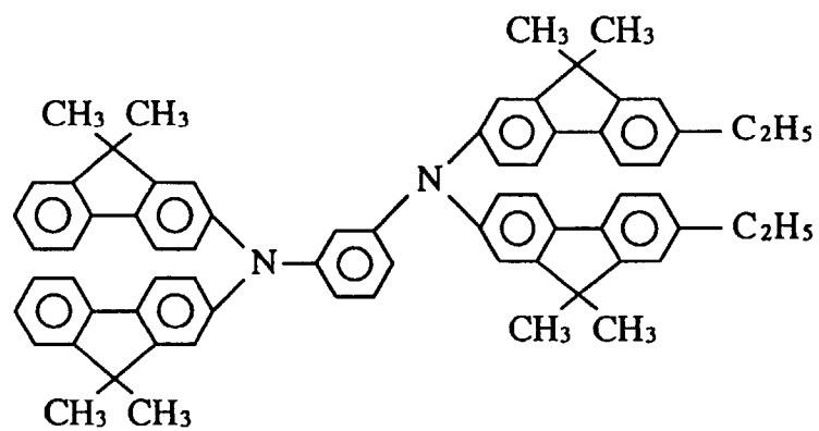
Compound 38
