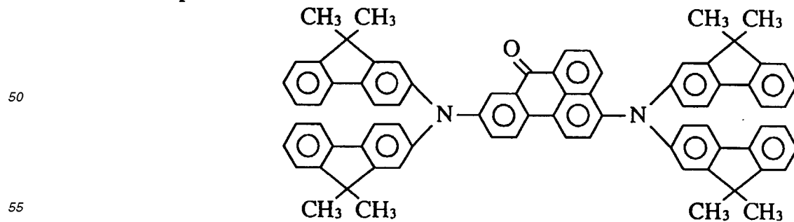
Compound 62
