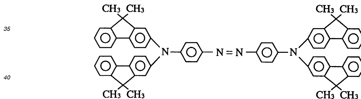
Compound 65
