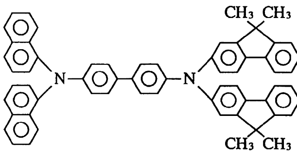
Compound 75
