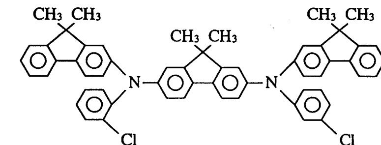
Compound 14
