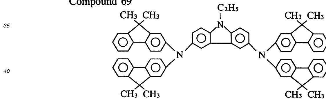
Compound 69
