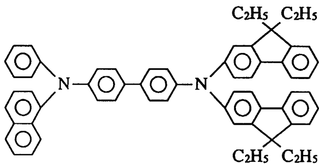
Compound 76
