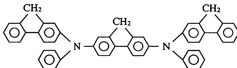
Compound 13
