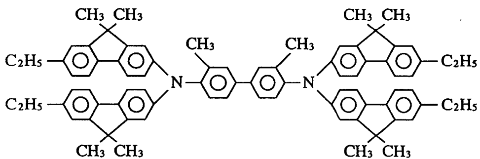
Compound 44
