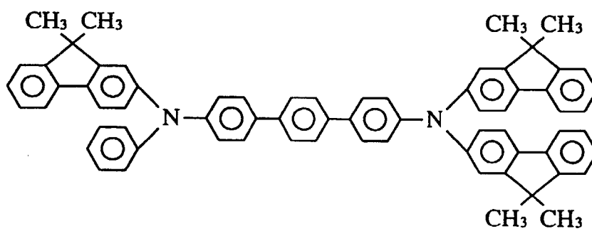
Compound 93
