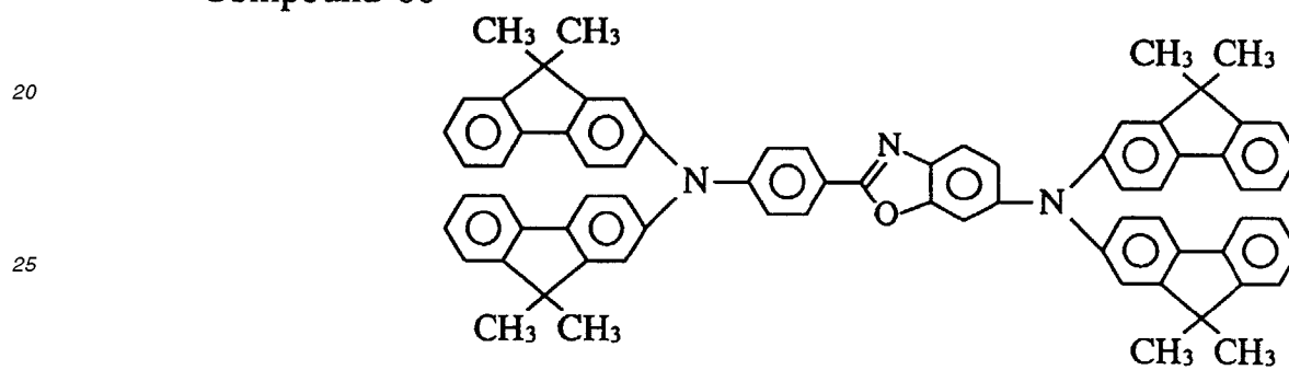
Compound 60
