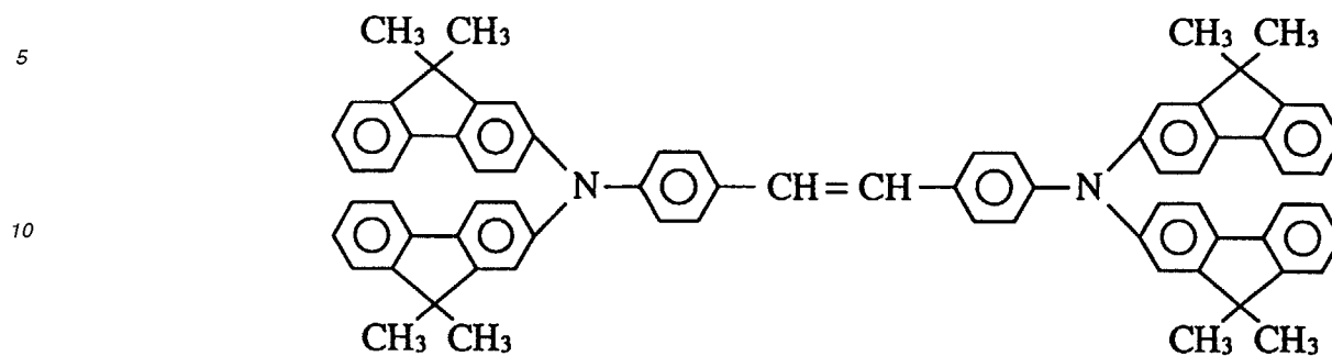
Compound 63
