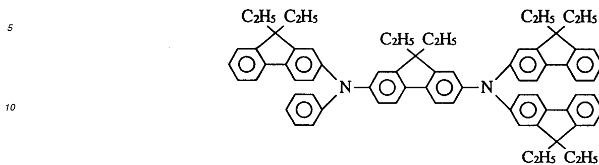
Compound 98
