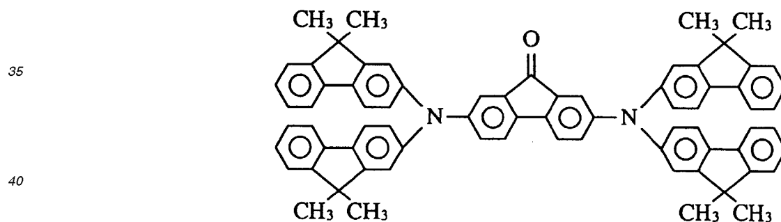
Compound 61
