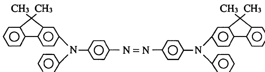
Compound 31
