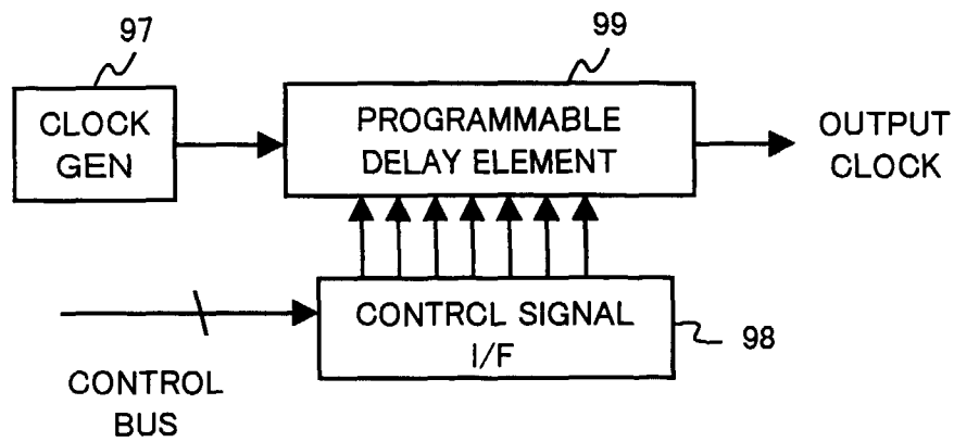
FIG. 29 (PRIOR ART)
