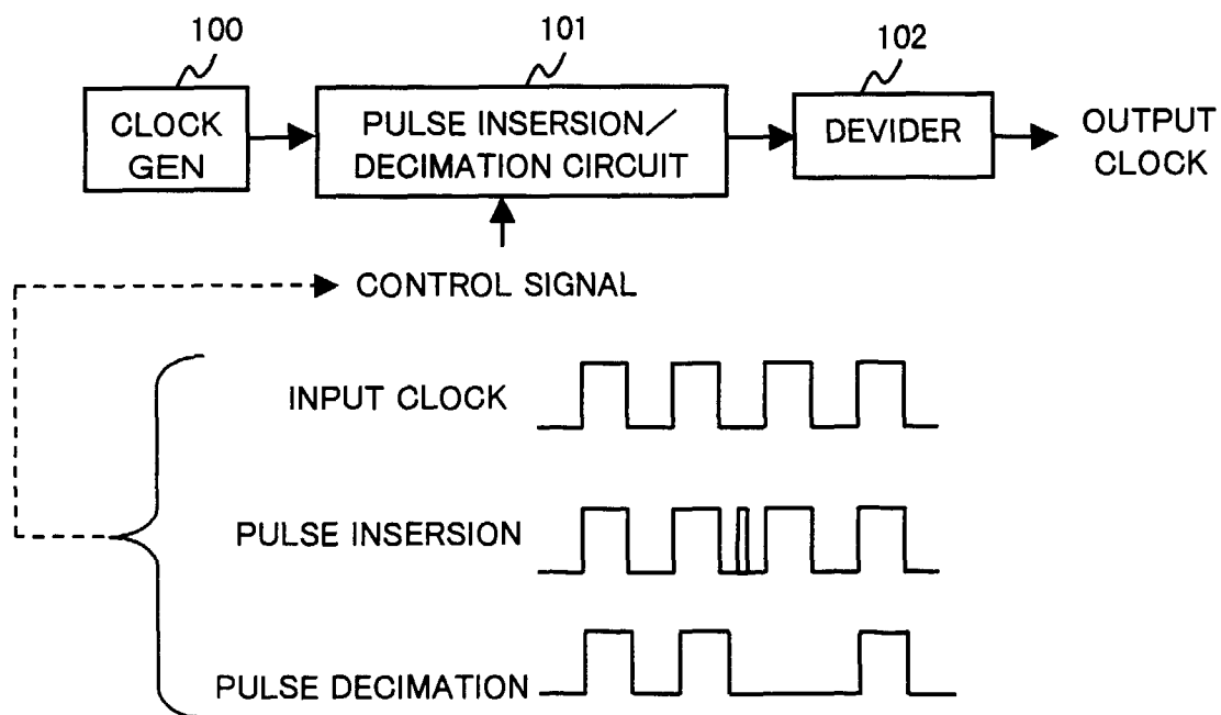
FIG. 30 (PRIOR ART)
