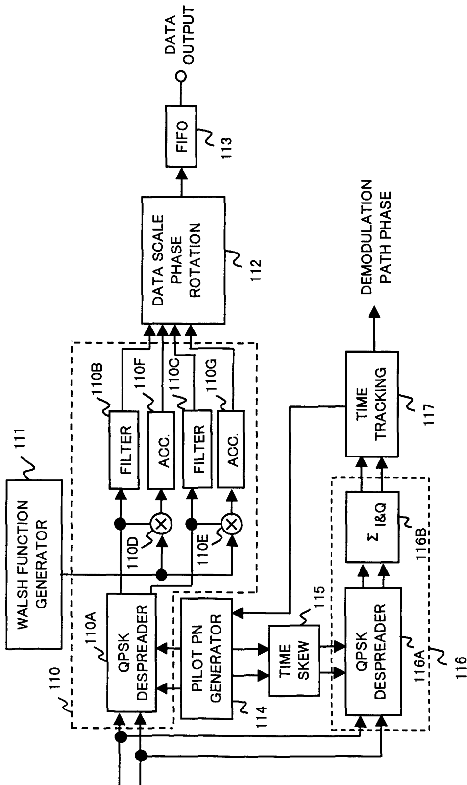
FIG. 32 (PRIOR ART)
