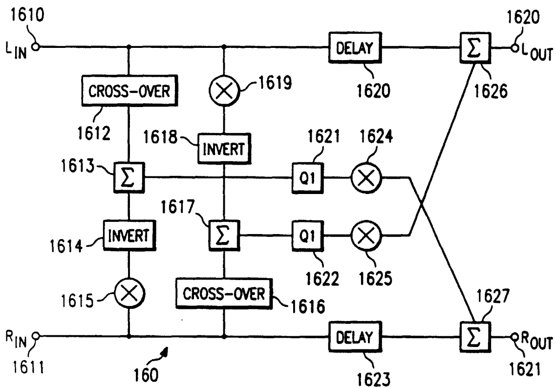
QX DUAL FILTER FIG. 8B (PRIOR ART)
