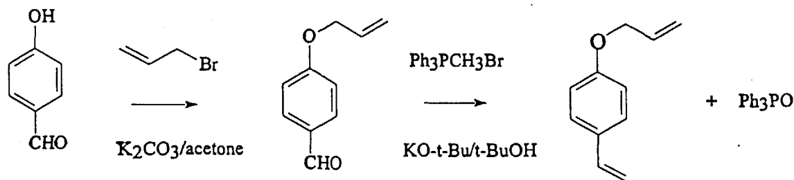
Scheme 1. Two stage synthesis of 4-allyloxystyrene by Wittig route
