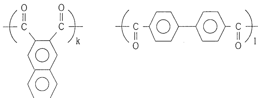
structural formula 14
