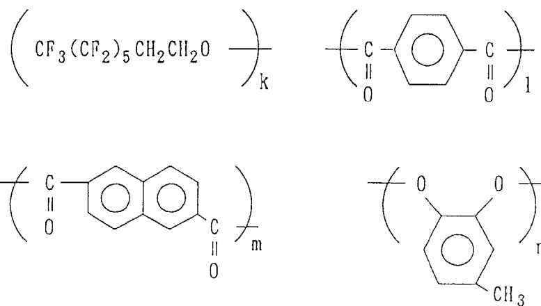
structural formula 38
