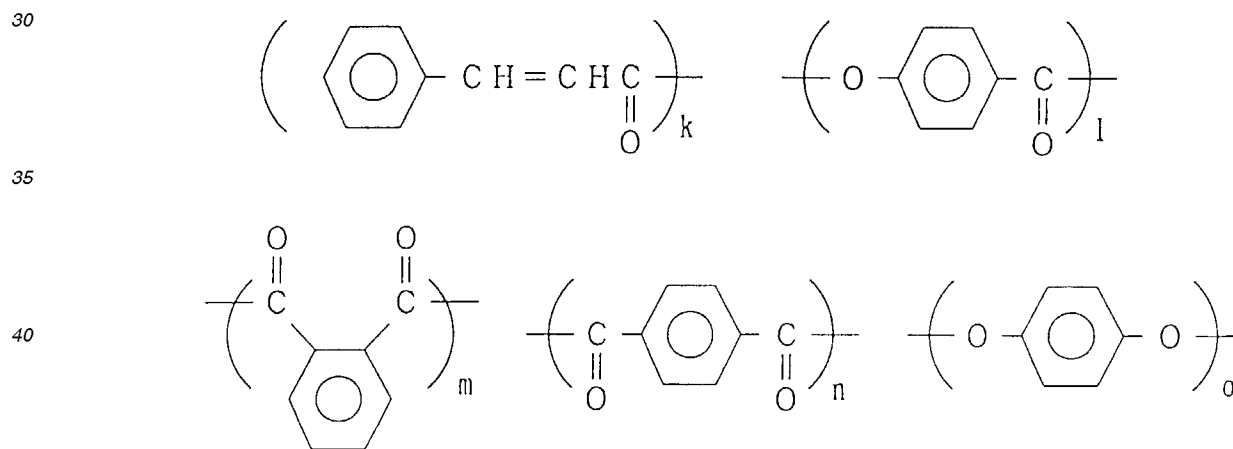
structural formula 74
