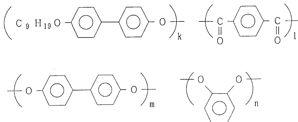
structural formula 30
