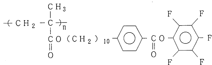
structural formula 53
