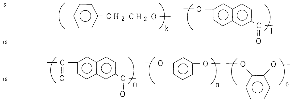
structural formula 73
