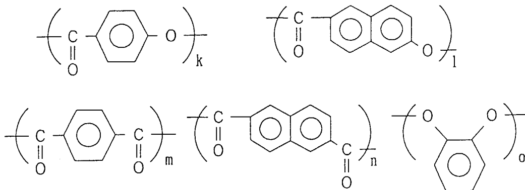
structural formula 64
