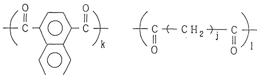
structural formula 15
