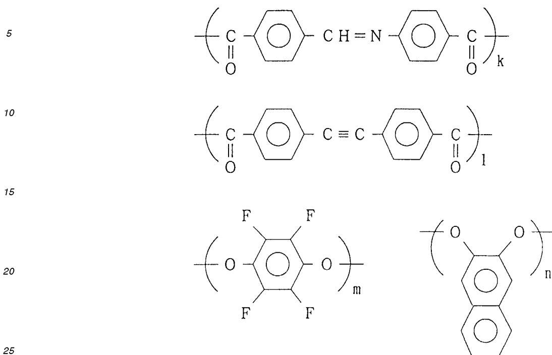
structural formula 18
