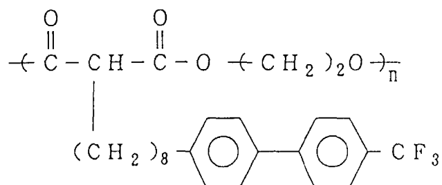
structural formula 59
