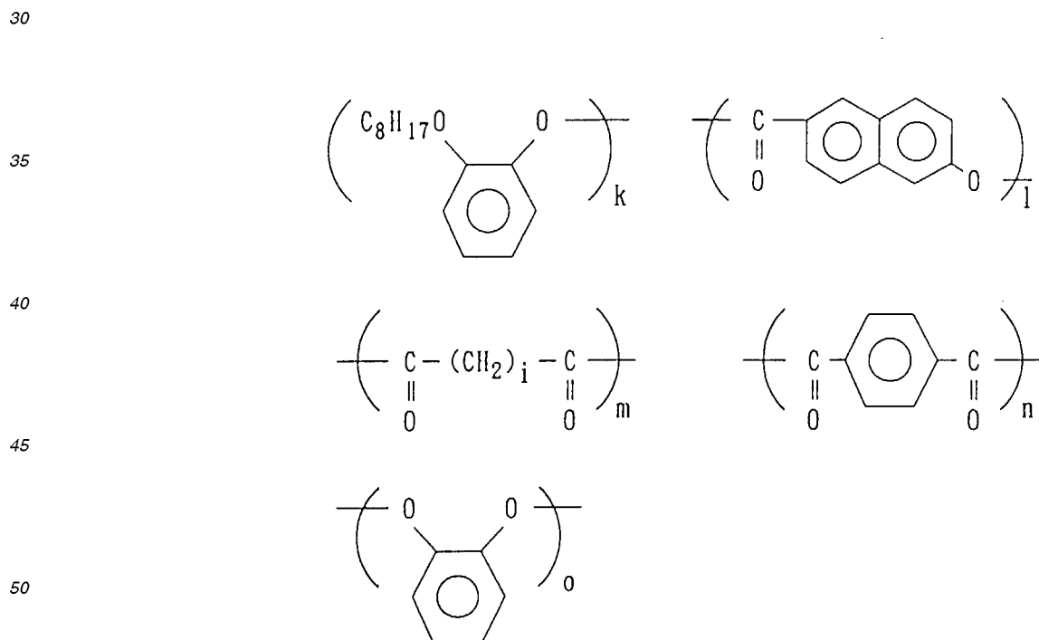
structural formula 33
