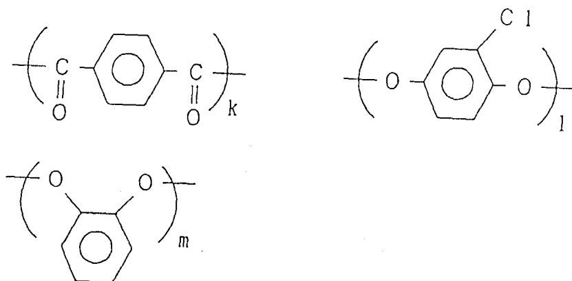
structural formula 63
