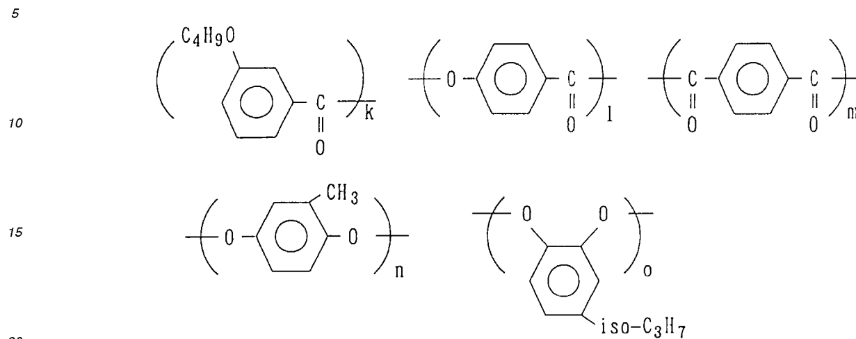
structural formula 32
