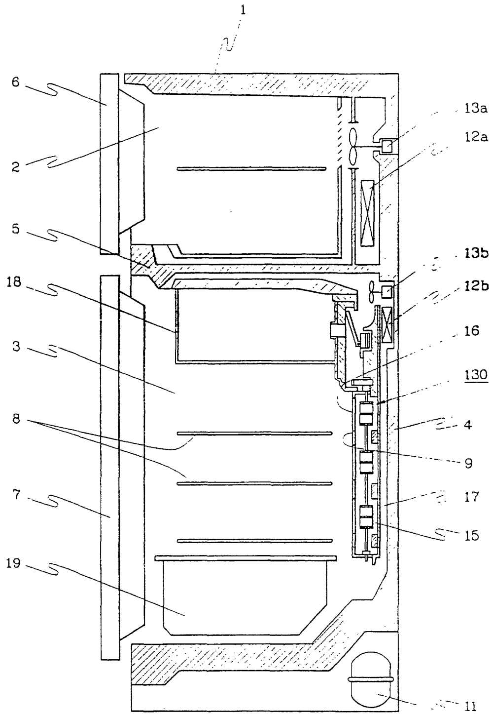
FIG. 1 (PRIOR ART)
