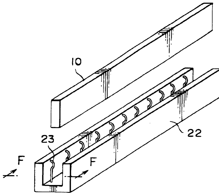
FIG. 4 PRIOR ART
