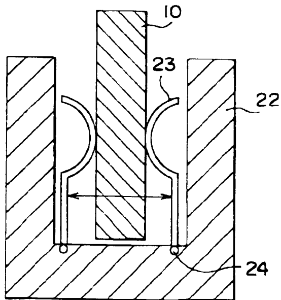
FIG. 5 PRIOR ART
