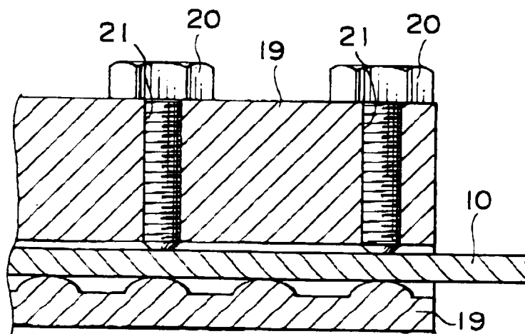
FIG. 3 PRIOR ART
