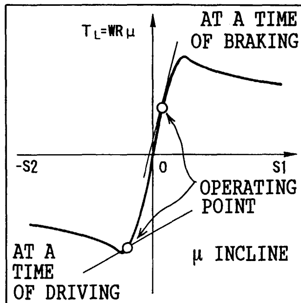
FRICTIONAL CHARACTERISTIC BETWEEN TIRE AND ROAD SURFACE
