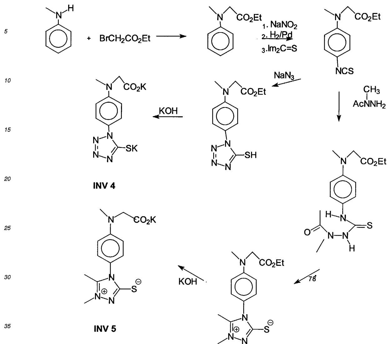
Scheme II
