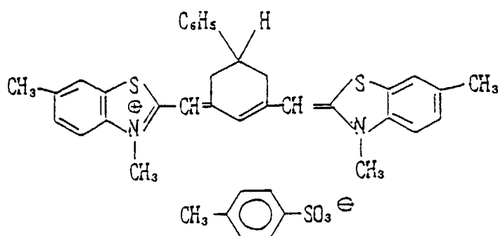
Sensitizing dye H
