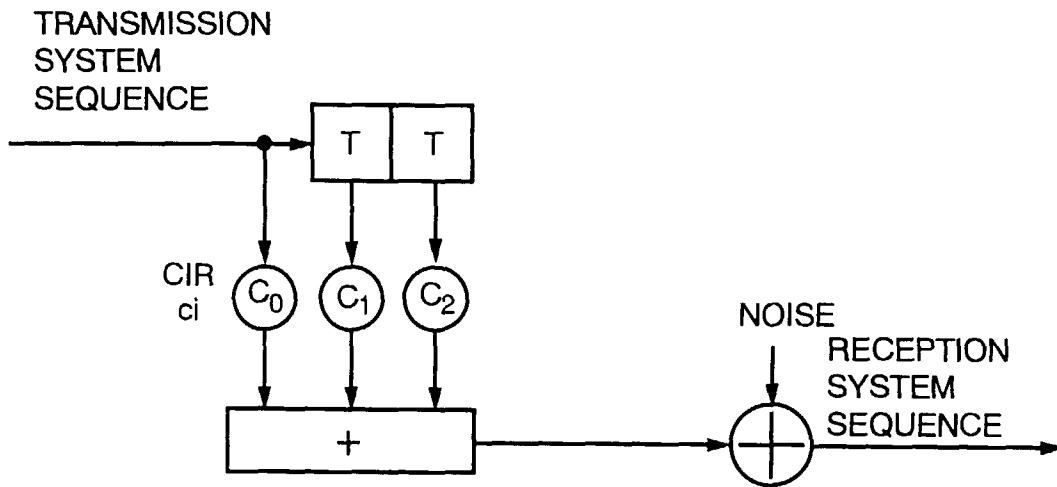
FIG. 18 (PRIOR ART)
