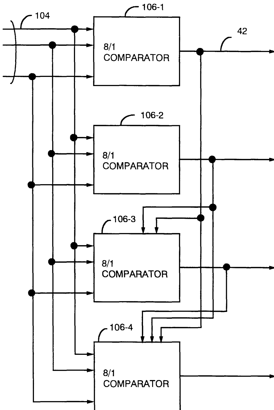
FIG. 27 (PRIOR ART)
