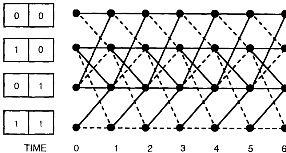
FIG. 19 (PRIOR ART)
