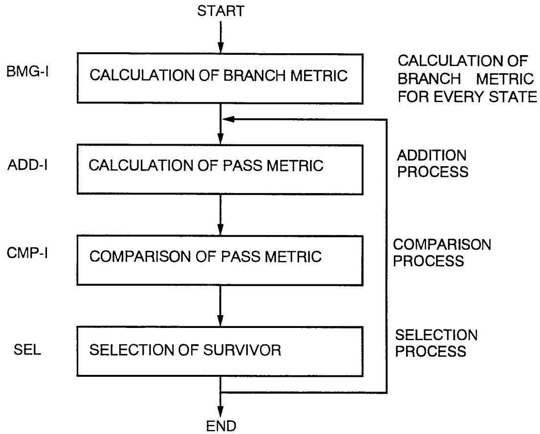
FIG. 20 (PRIOR ART)
