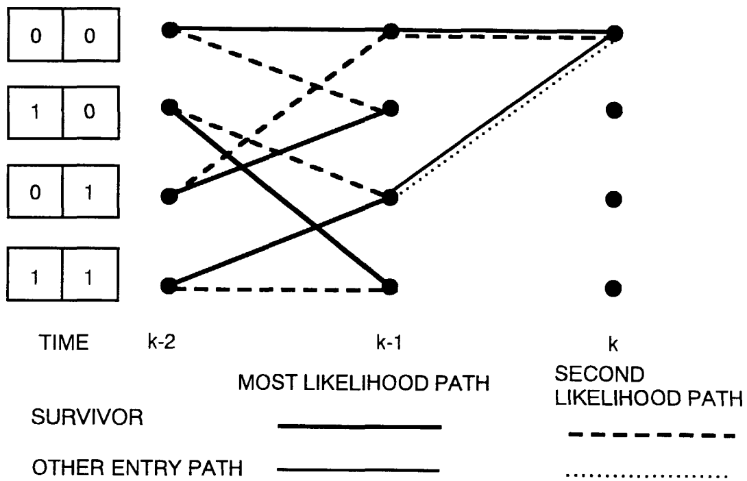
FIG. 24 (PRIOR ART)
