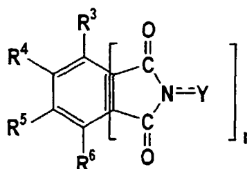
(1c)
