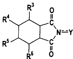
(1d)
