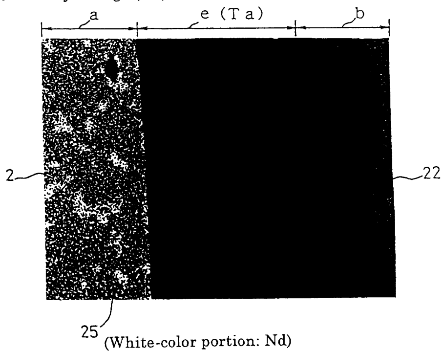
Characteristic X-rays image (Nd) Fig.15
