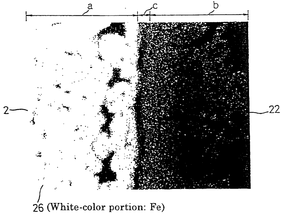
Fig. 9 Characteristic X-rays image (Fe)
