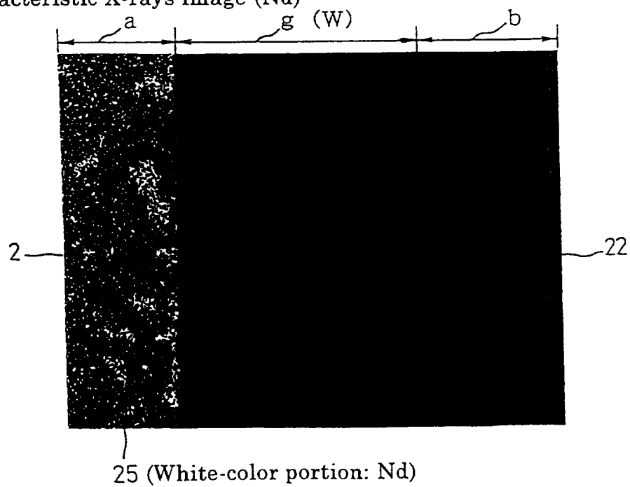
Fig.31 Characteristic X-rays image (Nd)
