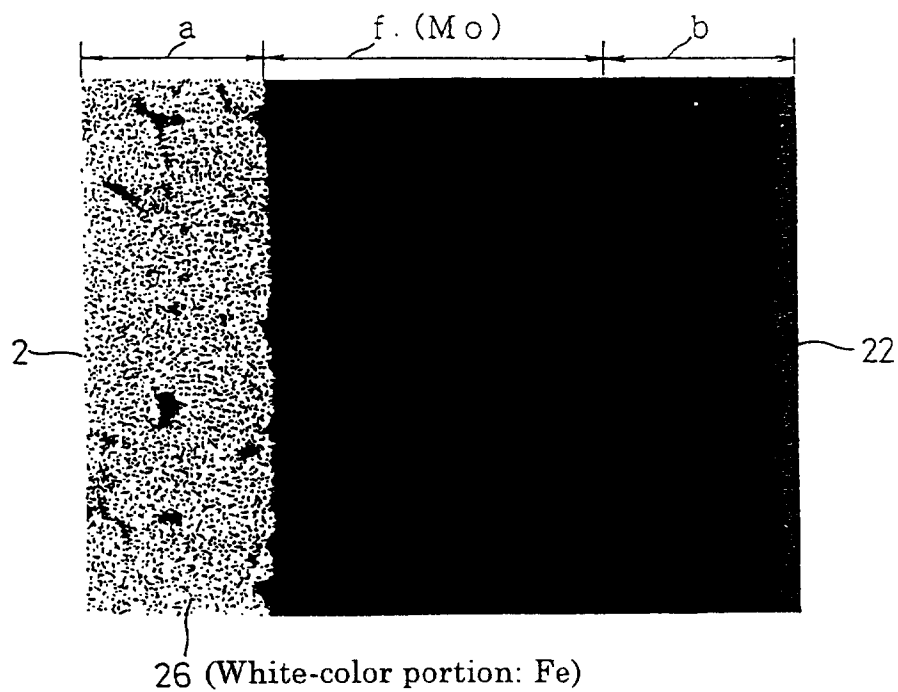
Fig. 24 Characteristic X-rays image (Fe)
