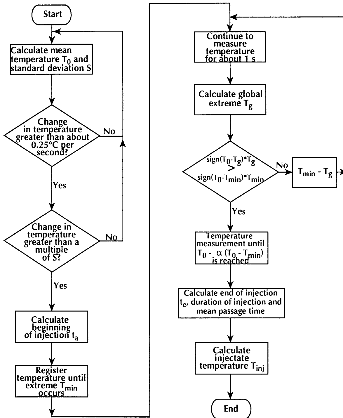
Flowchart for calculating the instant of injection, its duration and temperature.
