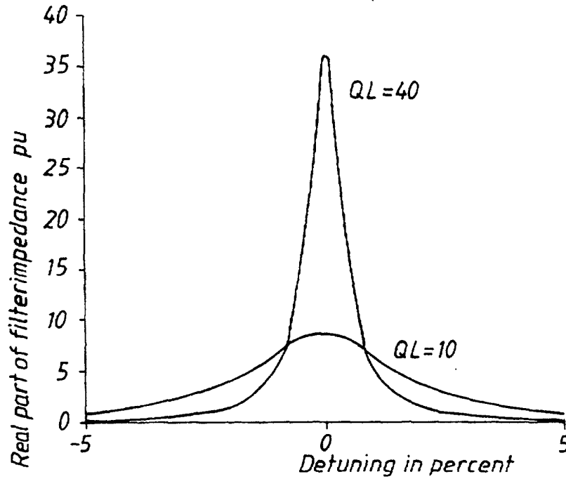
Real part of filter impedance, X_L=0.1 pu, Q_L=10 , Q_L=40
