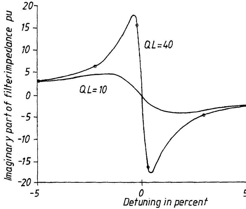
Imaginary part of filter impedance, X_L=0.1 pu, Q_L=10 , Q_L=40
