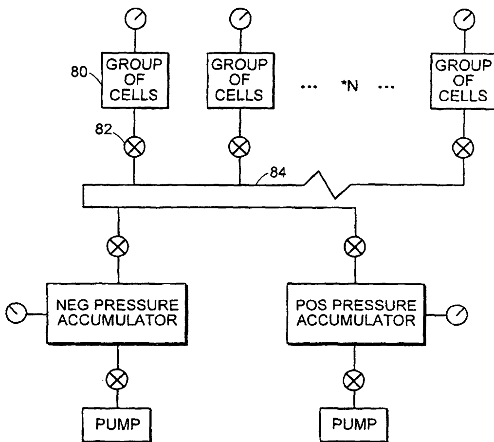
MODULAR CUSHION SCHEMATIC SINGLE ALTERNATING BUSS
