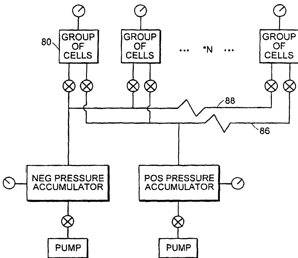
MODULAR CUSHION SCHEMATIC DUAL BUSS
