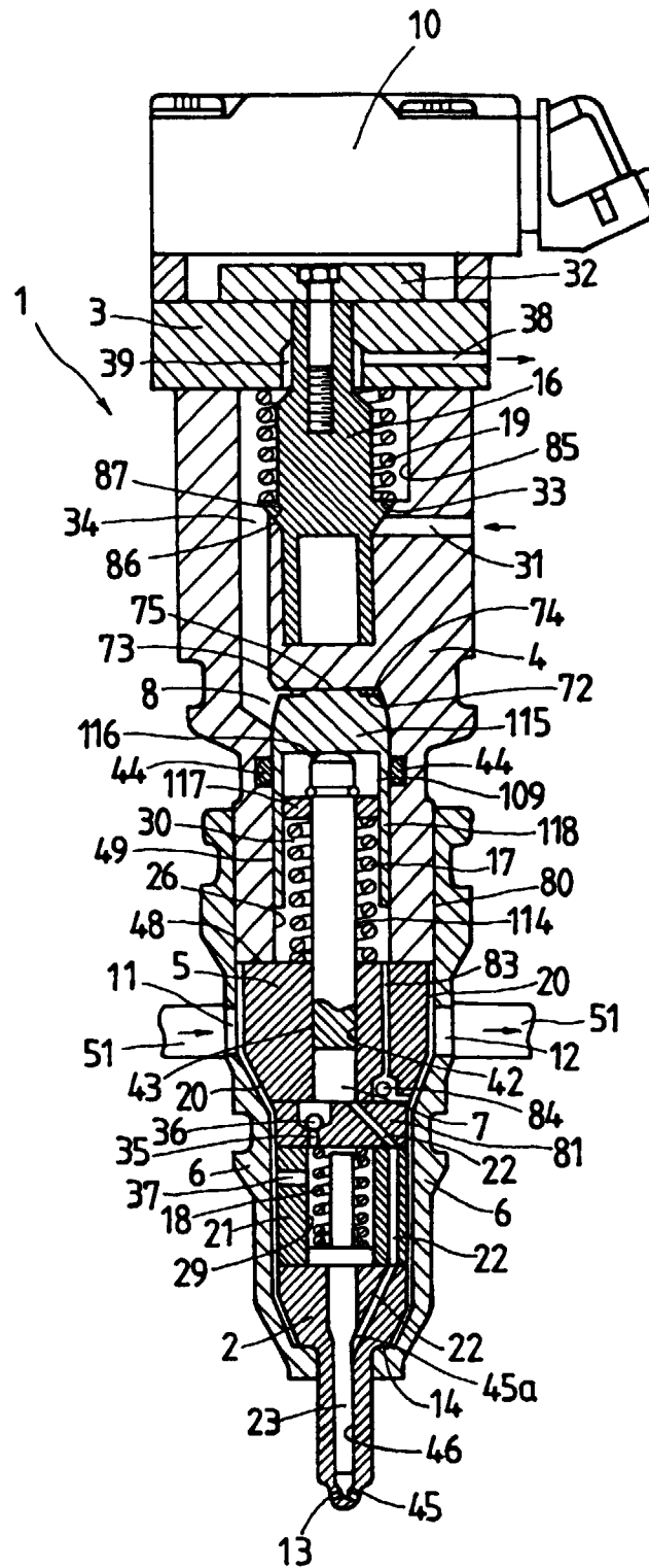
FIG. 13 (PRIOR ART)
