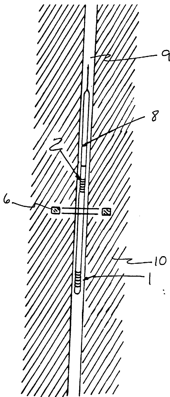
FIG. 2 (PRIOR ART)
