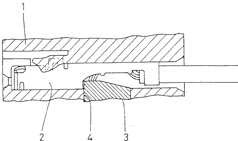
FIG. 8 PRIOR ART
