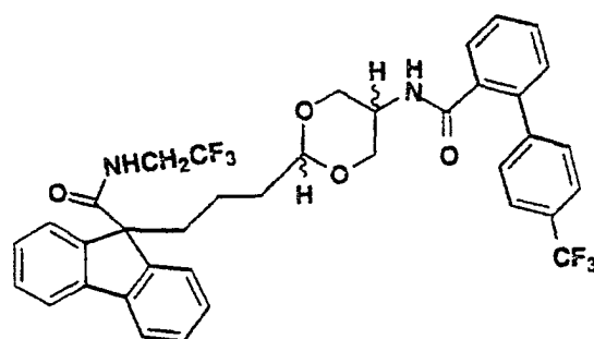
Isomer A
