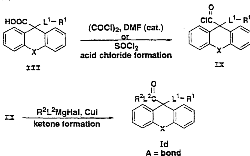
Scheme 4A
