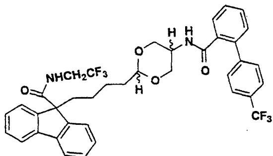
Isomer A
