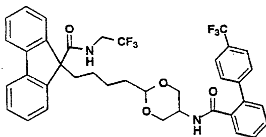
"Isomer B"
