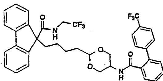
ISOMERE A
