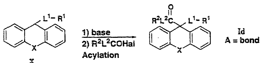
Scheme 4B
