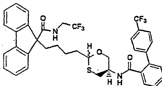
ISOMER A
