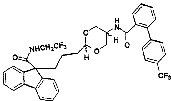
Isomer B
