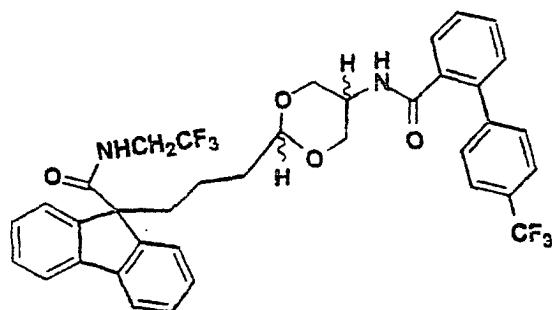
Isomer A
