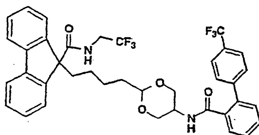
"Isomer A"
