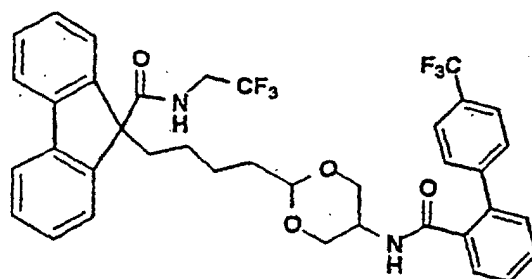
"Isomer B"
