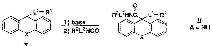
Scheme 8B
