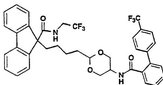
"Isomer A"
