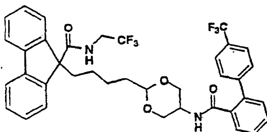
ISOMERE B
