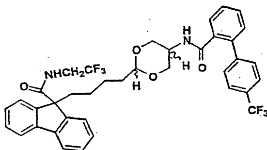
Isomer B
