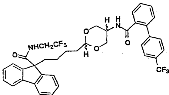
Isomer A
