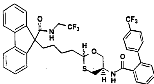
ISOMER A
