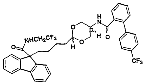
Isomer B
