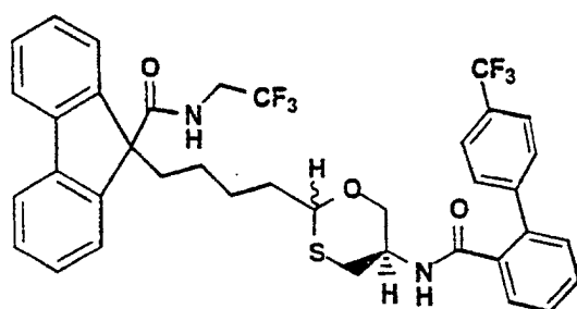
ISOMER B
