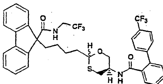
ISOMER B
