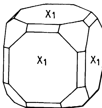
POLYHEDRON 1
