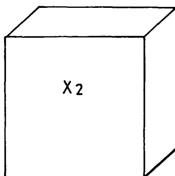
POLYHEDRON 2 (HEXAHEDRON)
