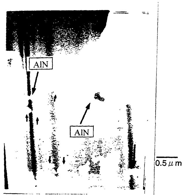
SINTERED ALUMINUM ALLOY FORMED BY DIRECT NITRIDING (TEM IMAGE)
