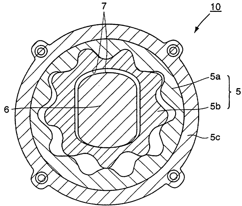
INSCRIBED GEAR ROTOR SET
