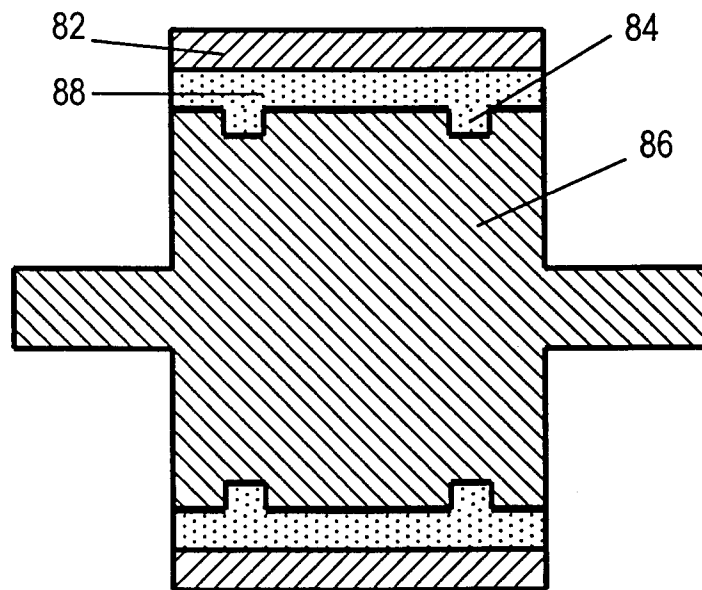
FIG.10 PRIOR ART
