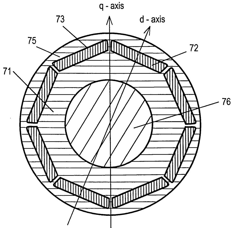
FIG.9 PRIOR ART
