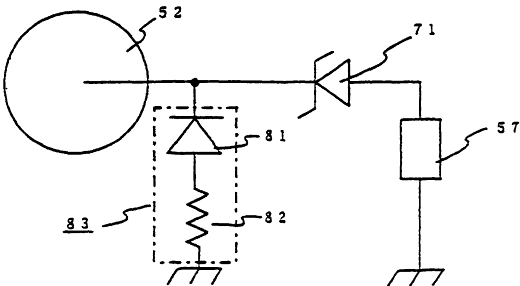
FIG. 8 PRIOR ART
