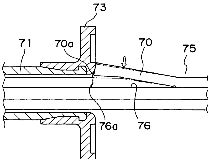
Fig.19 PRIOR ART
