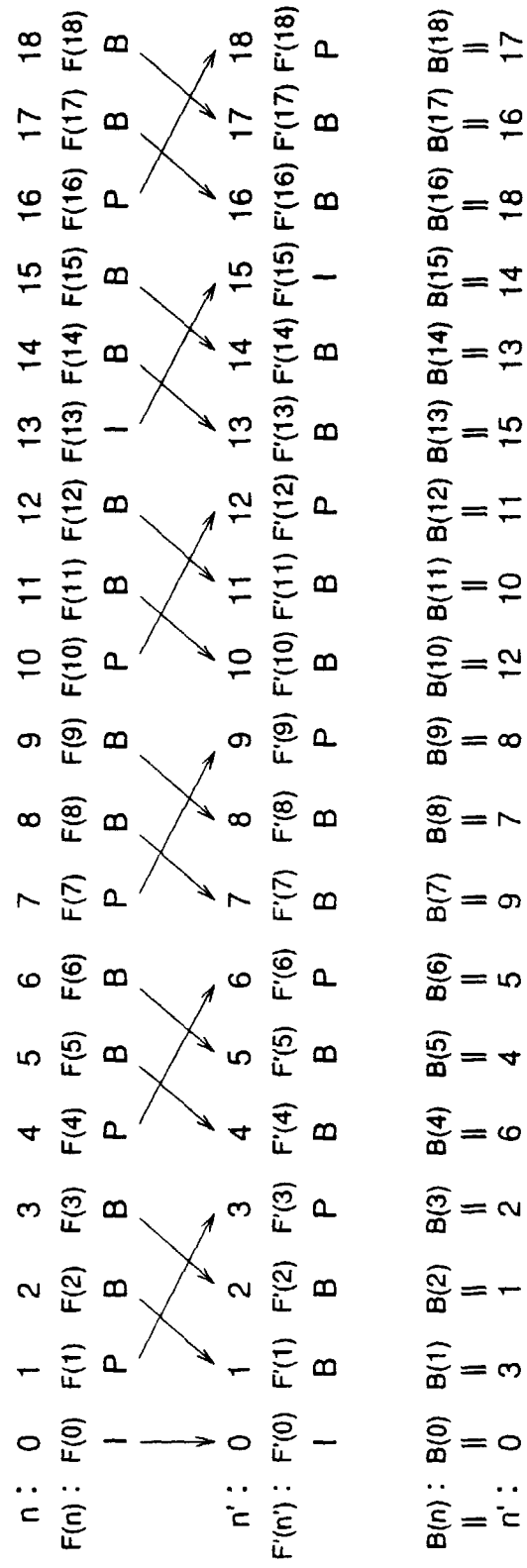
Fig.15 Prior Art
