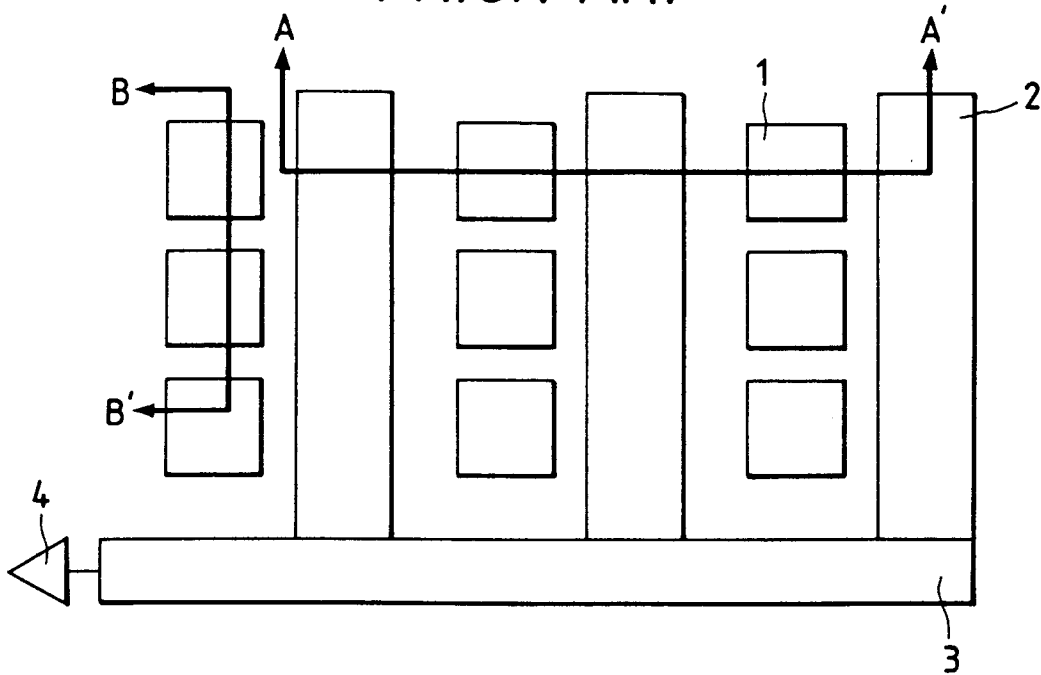
FIG. 24 PRIOR ART
