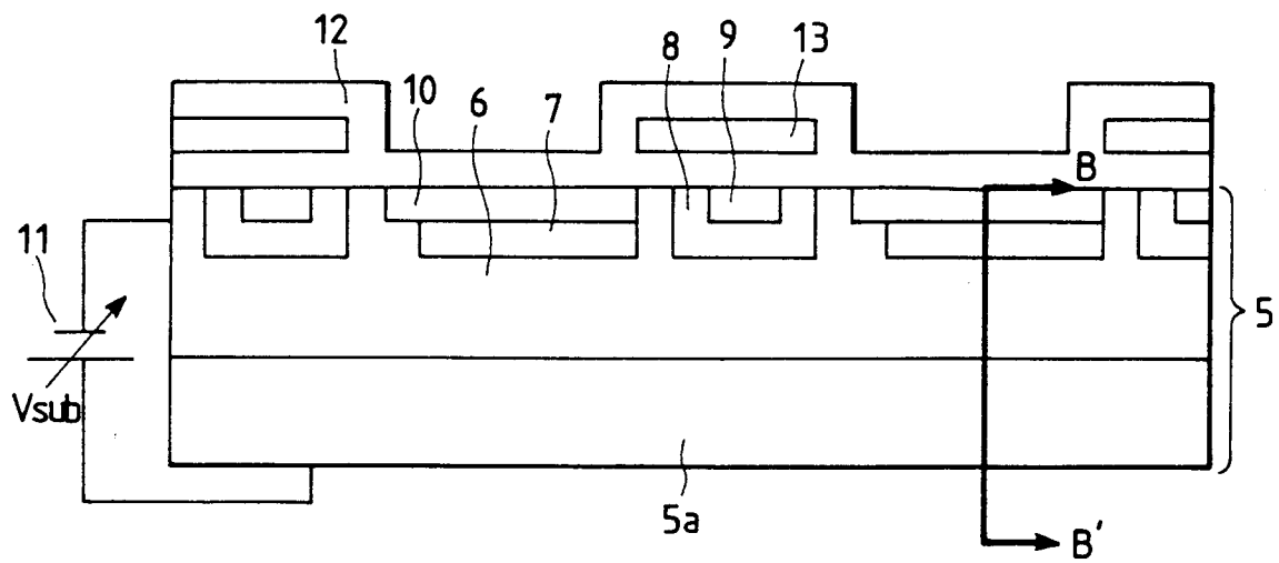
FIG. 25 PRIOR ART
