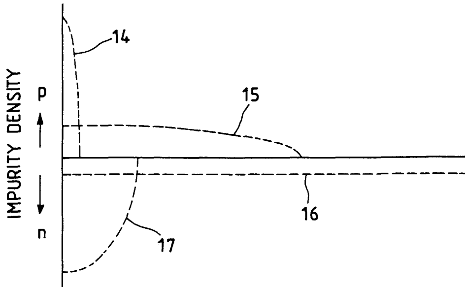
FIG. 26 PRIOR ART
