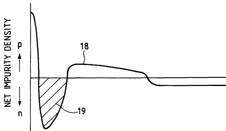
FIG. 27 PRIOR ART
