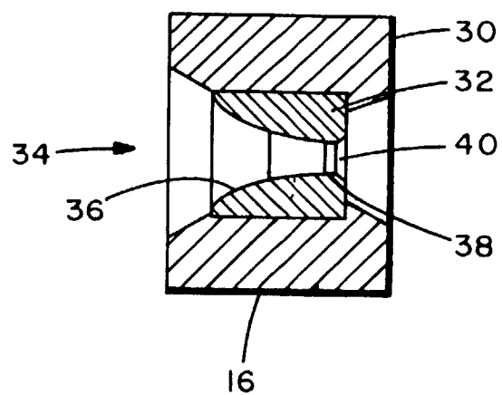
FIG. 2 (PRIOR ART)
