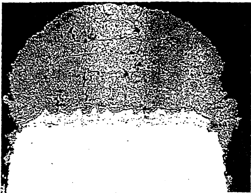
b. A31(1) X100 Panel: As Tested
