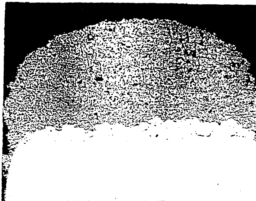
a. A31(1) X100 Panel: As Sprayed
