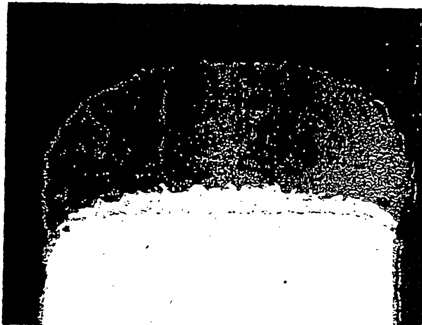
b. A31(2) X75 Blade: As Tested
