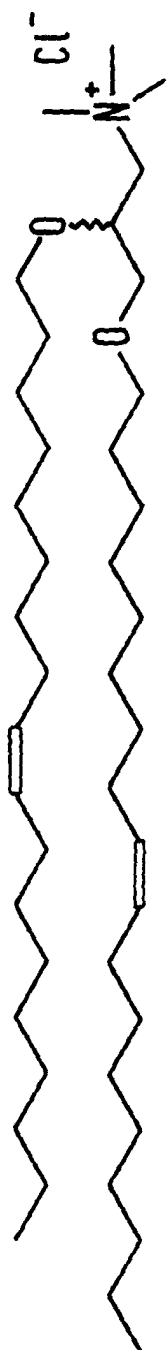
DOTMA N -[1-(2,3-dioleoyloxy)propyl]- N,N,N -trimethyl ammonium chloride
