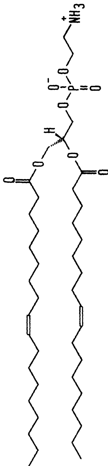
DOPE Dioleoylphosphatidyl ethanolamine
