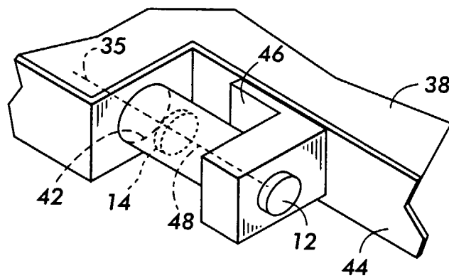
FIG. 2 ( Prior Art )
