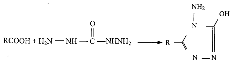
thiocarbohydrazide
