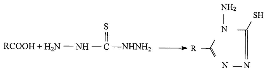
thiocarbohydrazide
