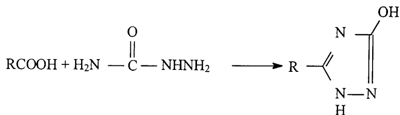
3-hydroxytriazole
