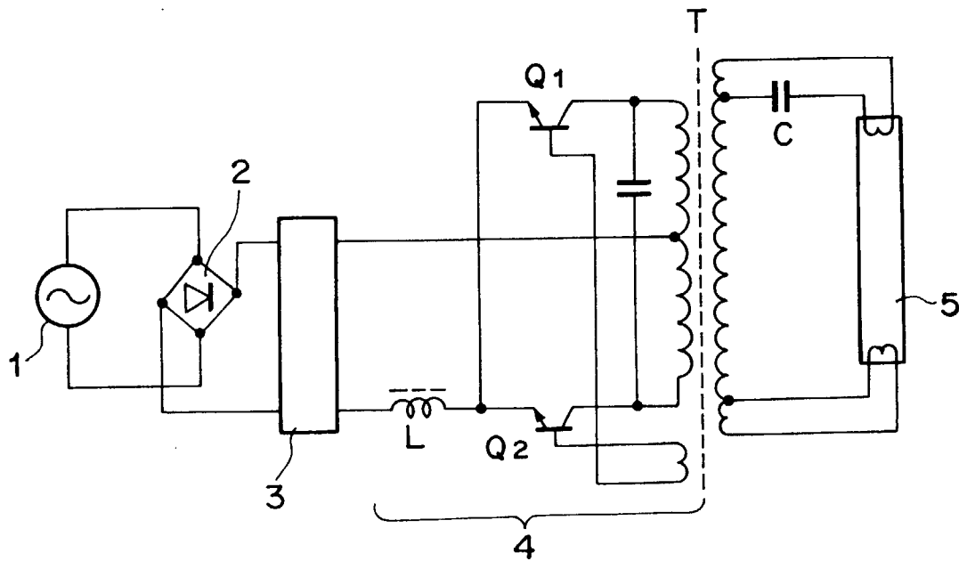
FIG. 21 PRIOR ART
