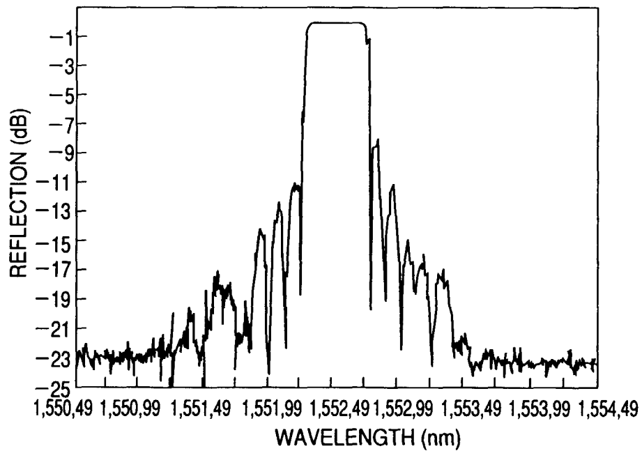
32 REFLECTION CHARACTERISTIC
