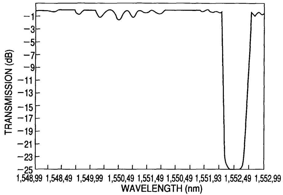
31 TRANSMISSION CHARACTERISTIC
