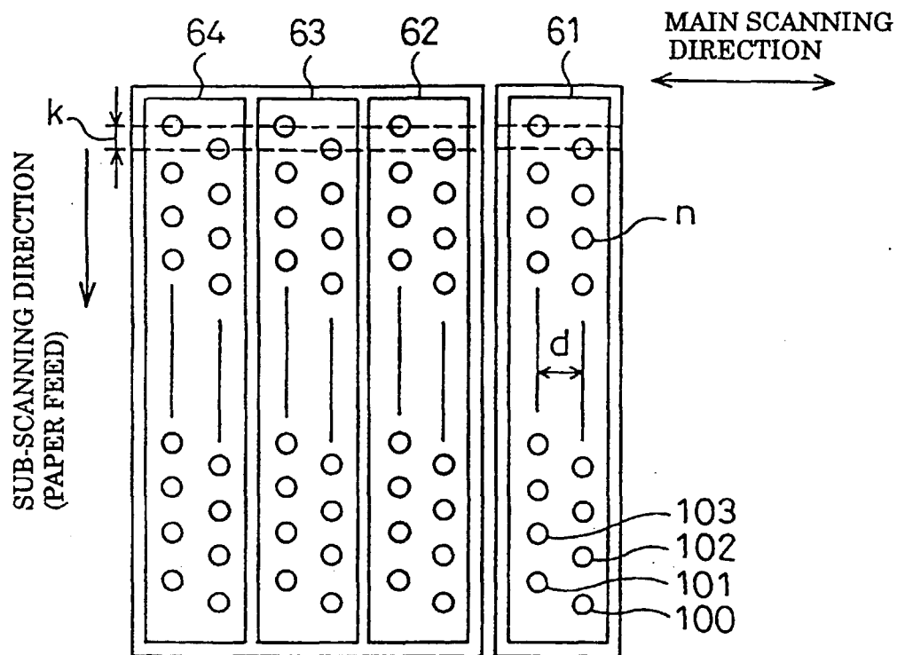
Fig. 5 (B) DOTS FORMED BY ONE NOZZLE ARRAY
