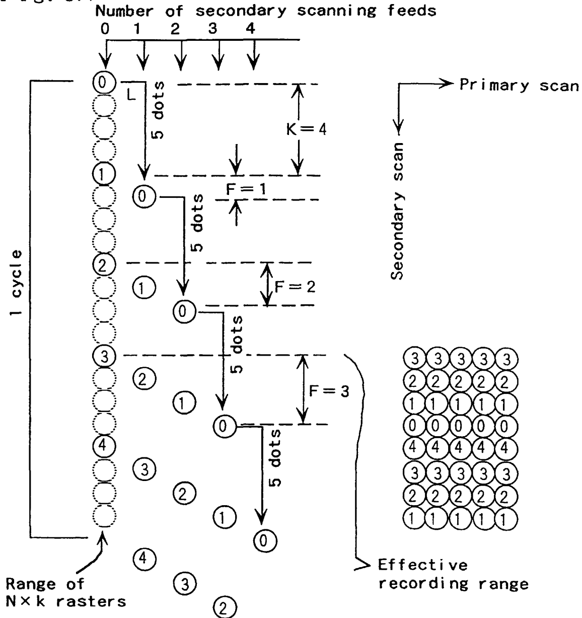
Fig. 9A CONCEPT OF SECONDARY SCANNING FEED
