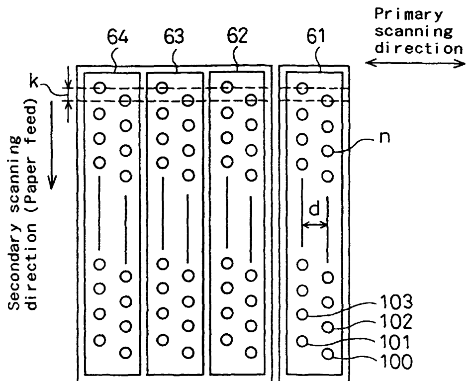
Fig. 8B DOTS FORMED BY ONE NOZZLE ARRAY
