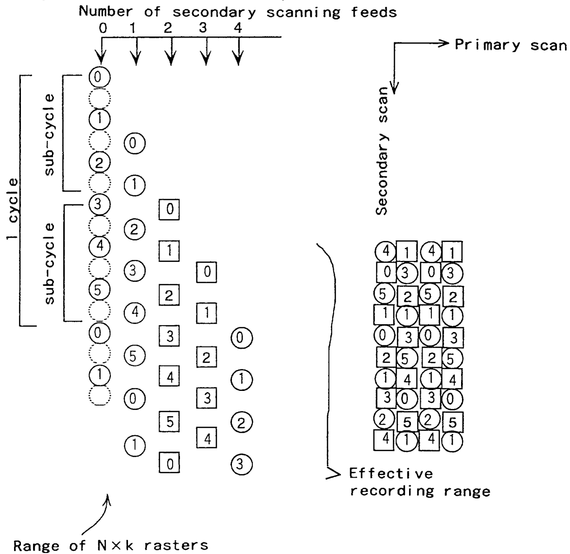
Fig. 19A CONCEPT OF SECONDARY SCANNING FEED
